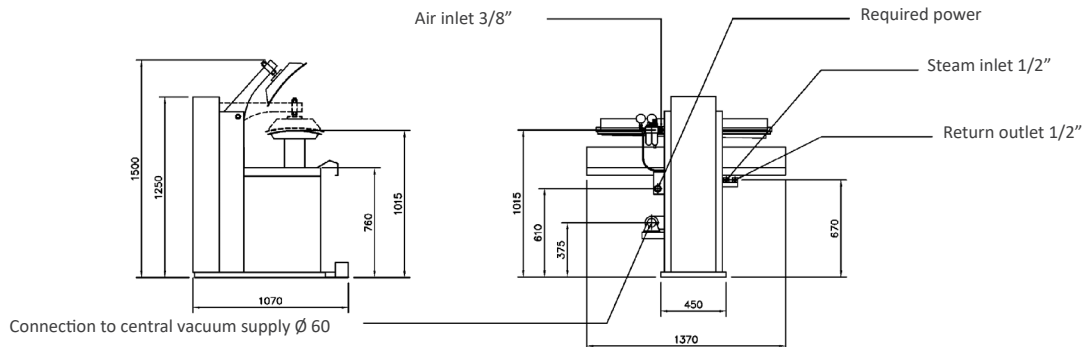
PRESS WITHOUT BOILER
